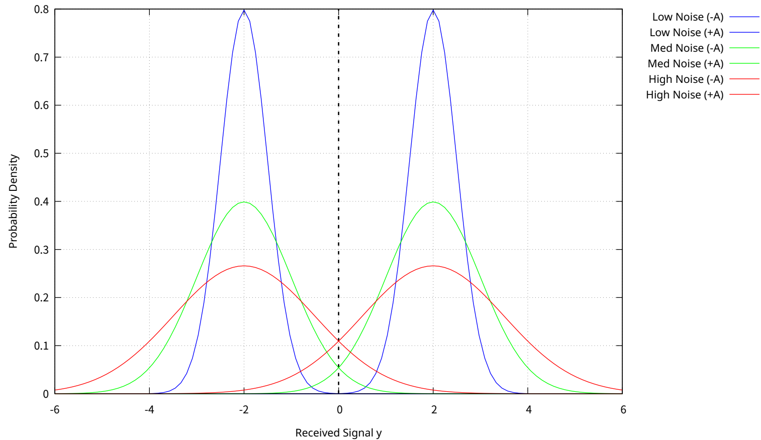
BPSK Signal Overlap with Increasing Jamming Power
