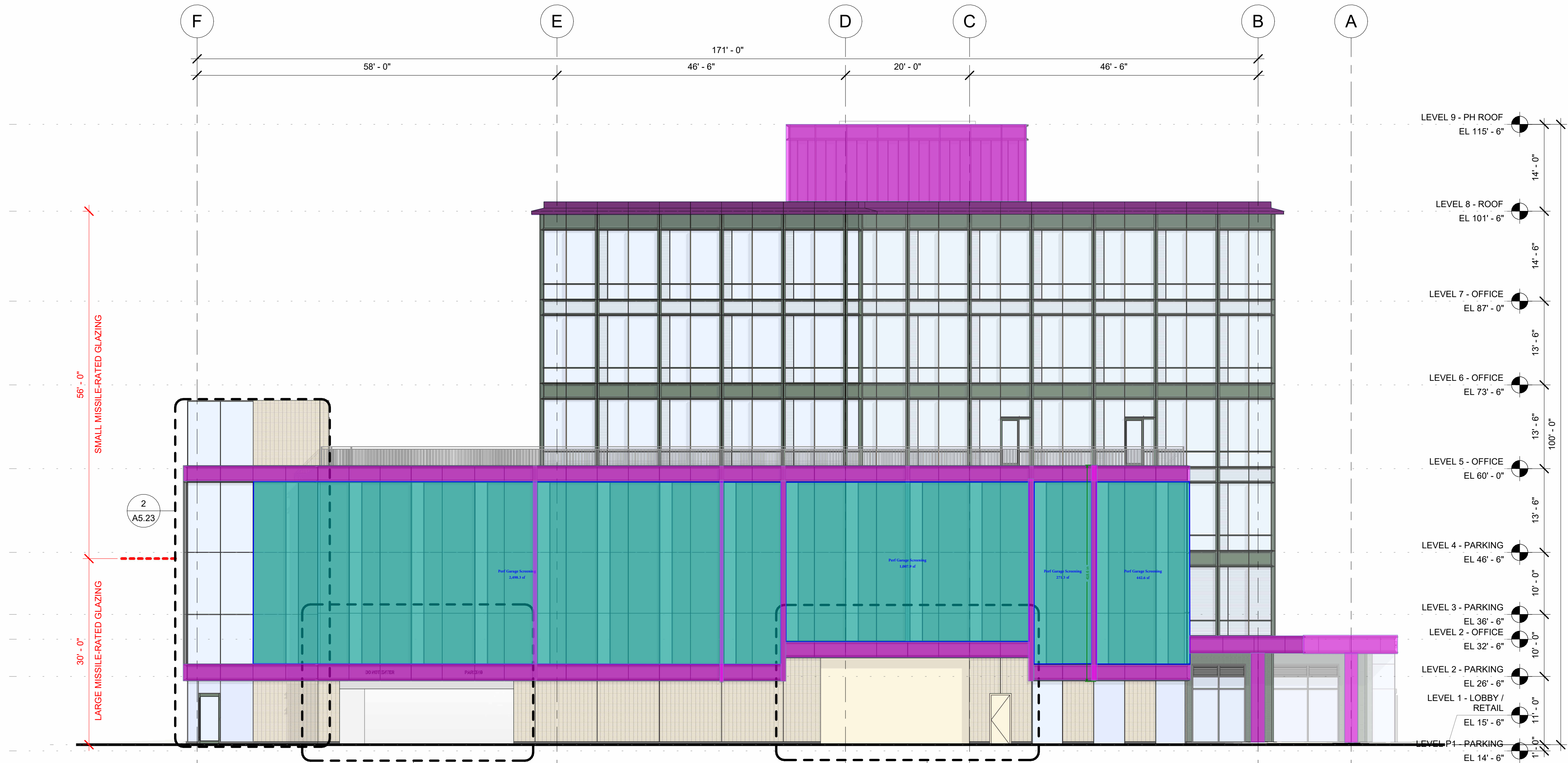
1 EAST ELEVATION 3/32" = 1'-0"
