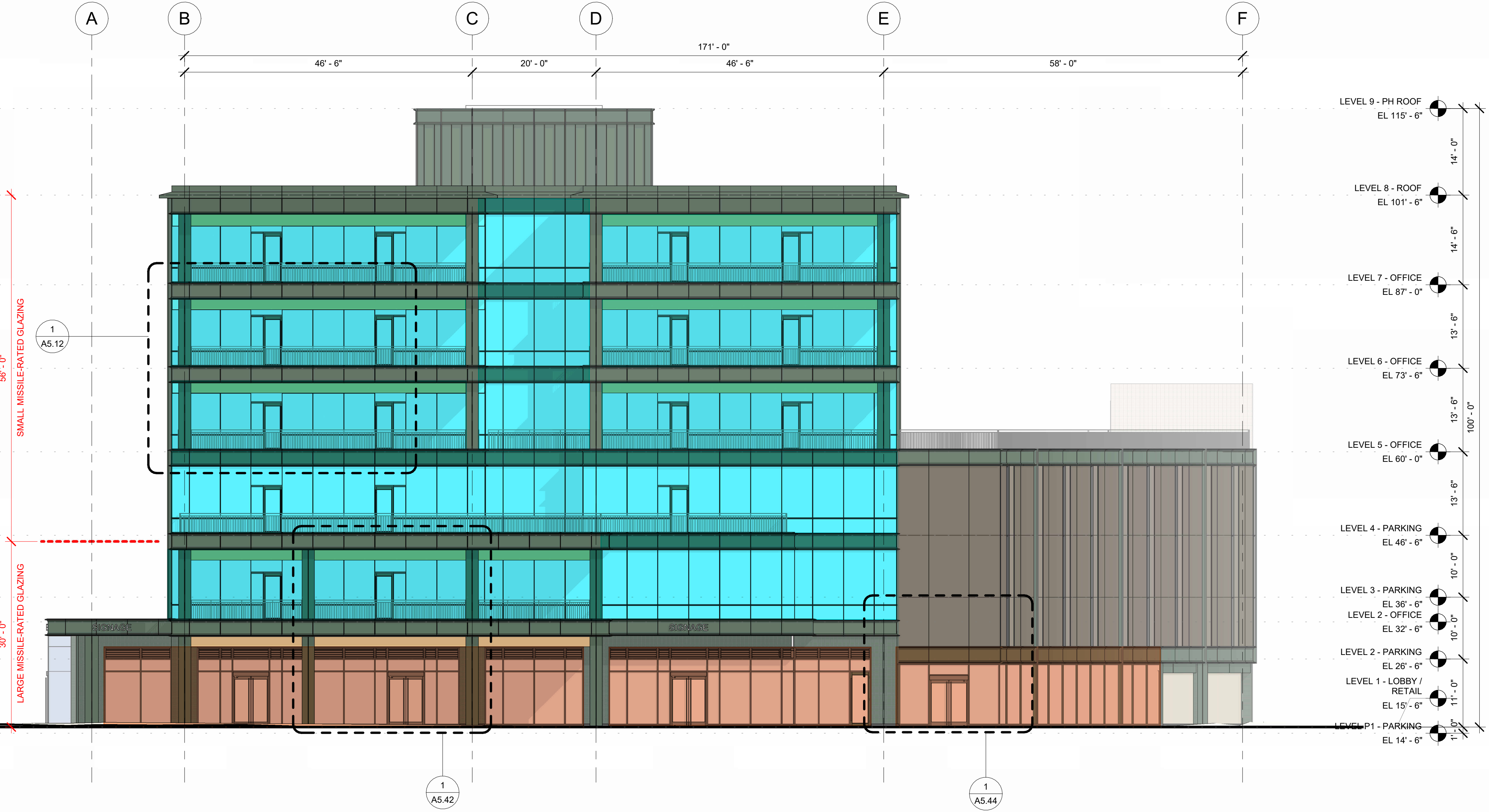
2 WEST ELEVATION 3/32" = 1'-0"
