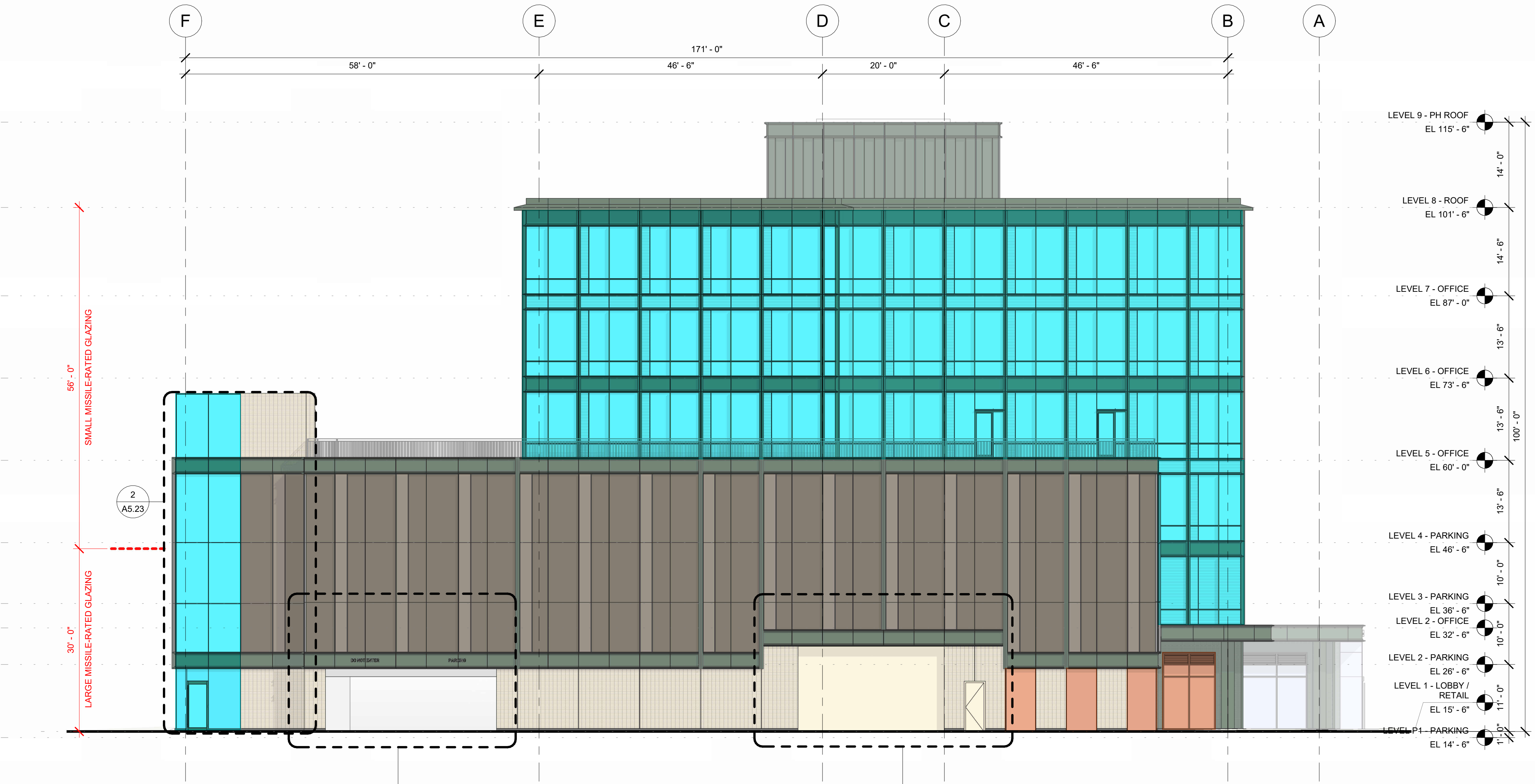
1 EAST ELEVATION 3/32" = 1'-0"
