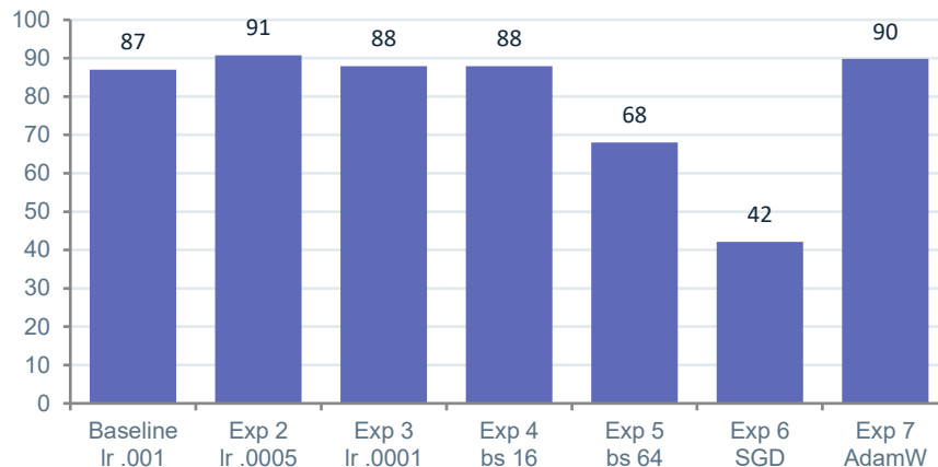
MobileNetV3 hyperparameter sweep (accuracy %)
