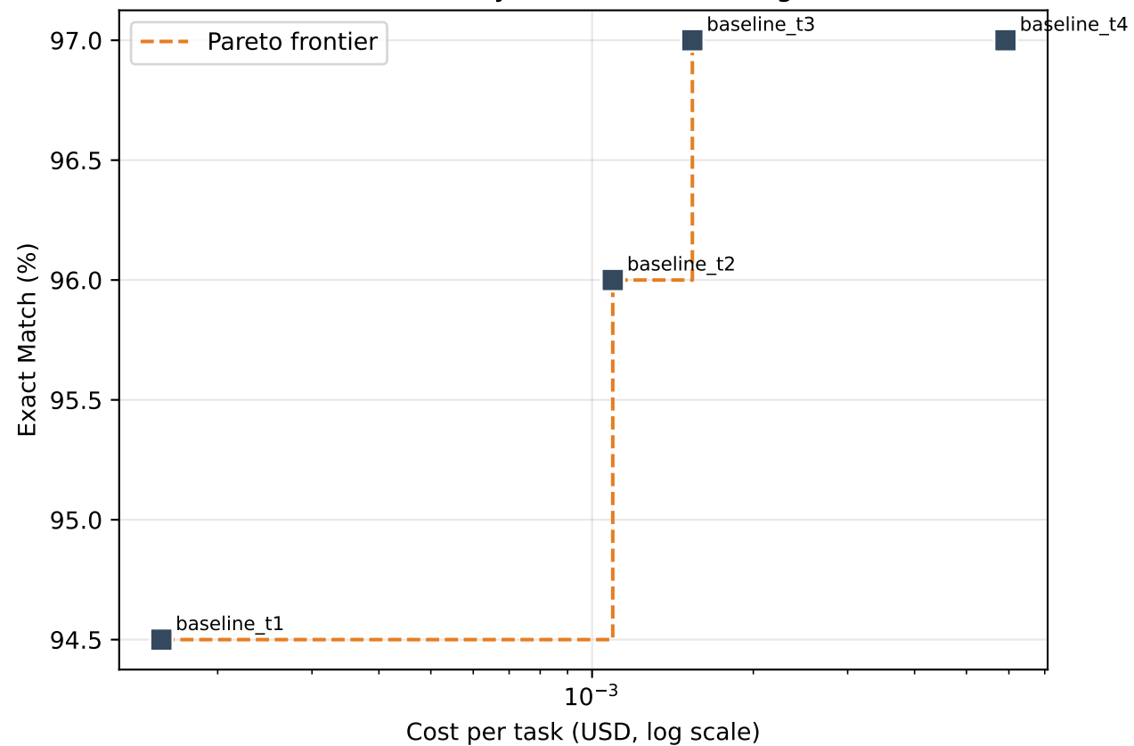
Cost vs Quality Pareto Frontier — gsm8k
