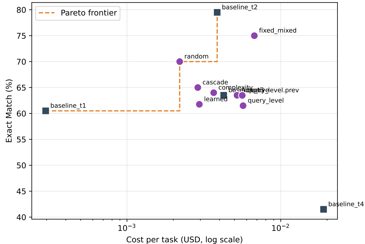
Cost vs Quality Pareto Frontier — hotpotqa
