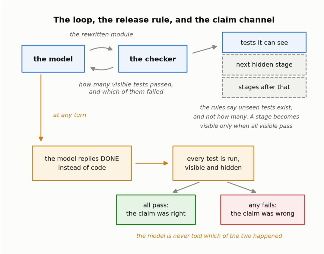
Figure 1: The harness loop, with the two things this paper adds to it. The hidden tests arrive in stages rather than all at once, and the model may end the episode by replying DONE, which is scored against the tests it has not seen and never reported back to it. Drawn by figures/make_figures.py: f1_harness_loop.
