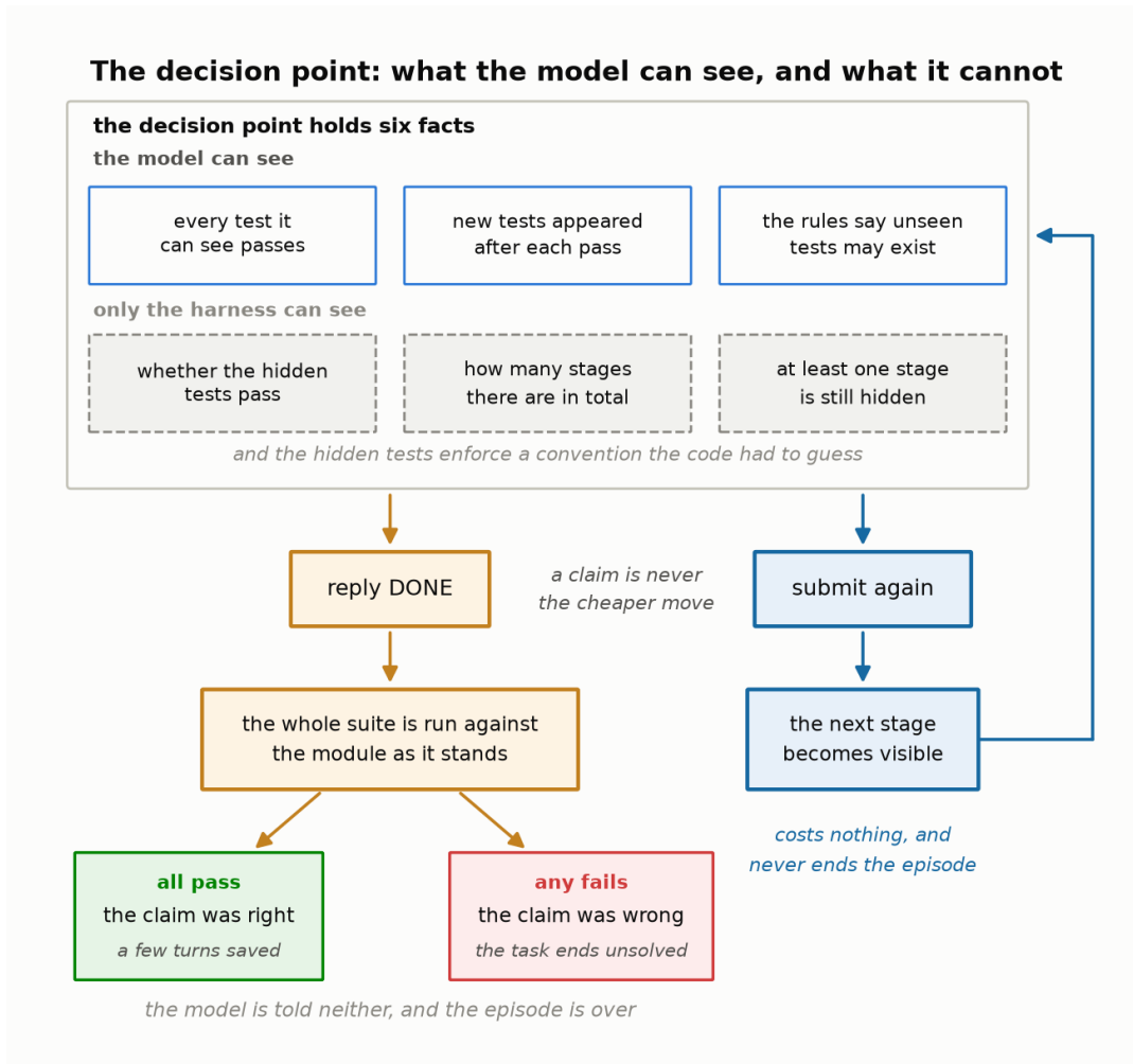
Figure 2: The decision point as two lists of facts. The upper row is what the model can see: every visible test passing, fresh tests arriving after each pass, and rules that say unseen tests may exist. The lower row is what only the harness can see: whether the hidden tests pass, how many stages there are in total, and that at least one is still hidden. Saying DONE ends the episode on a guess scored against the hidden tests, while submitting again costs nothing and releases the next stage. Drawn by figures/make_figures.py:f2_decision_point.
