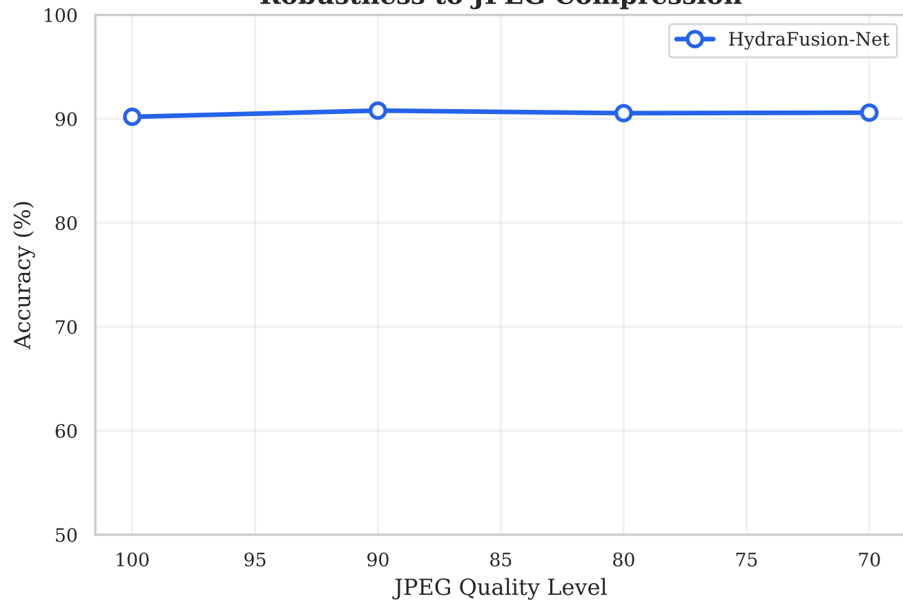
Robustness to JPEG Compression
