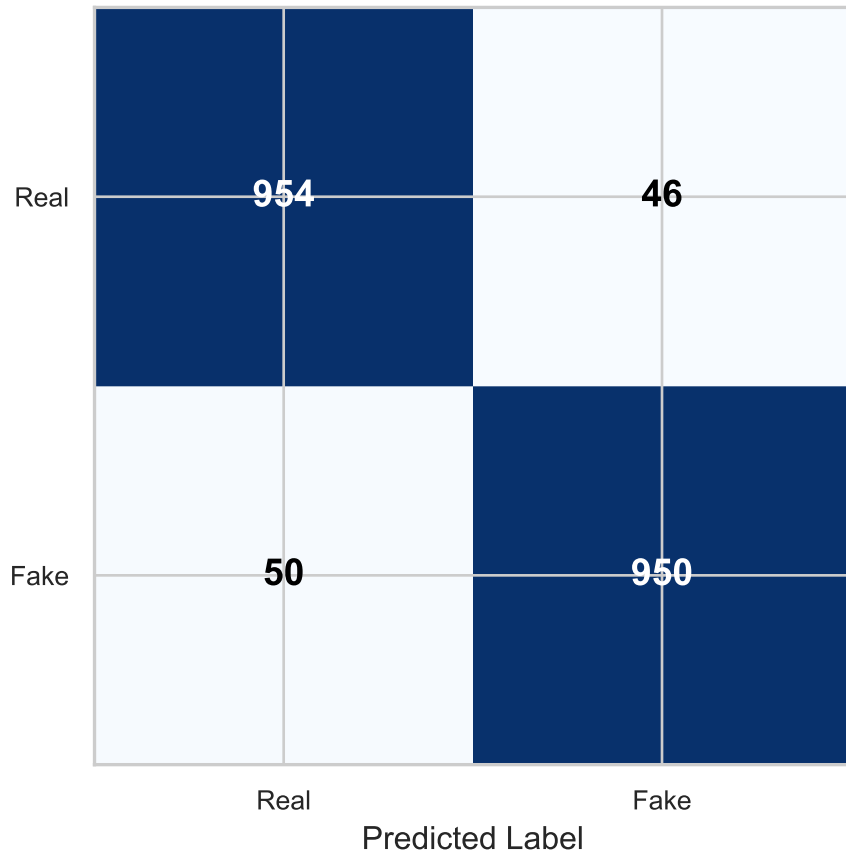
Confusion Matrix (Raw Counts)
