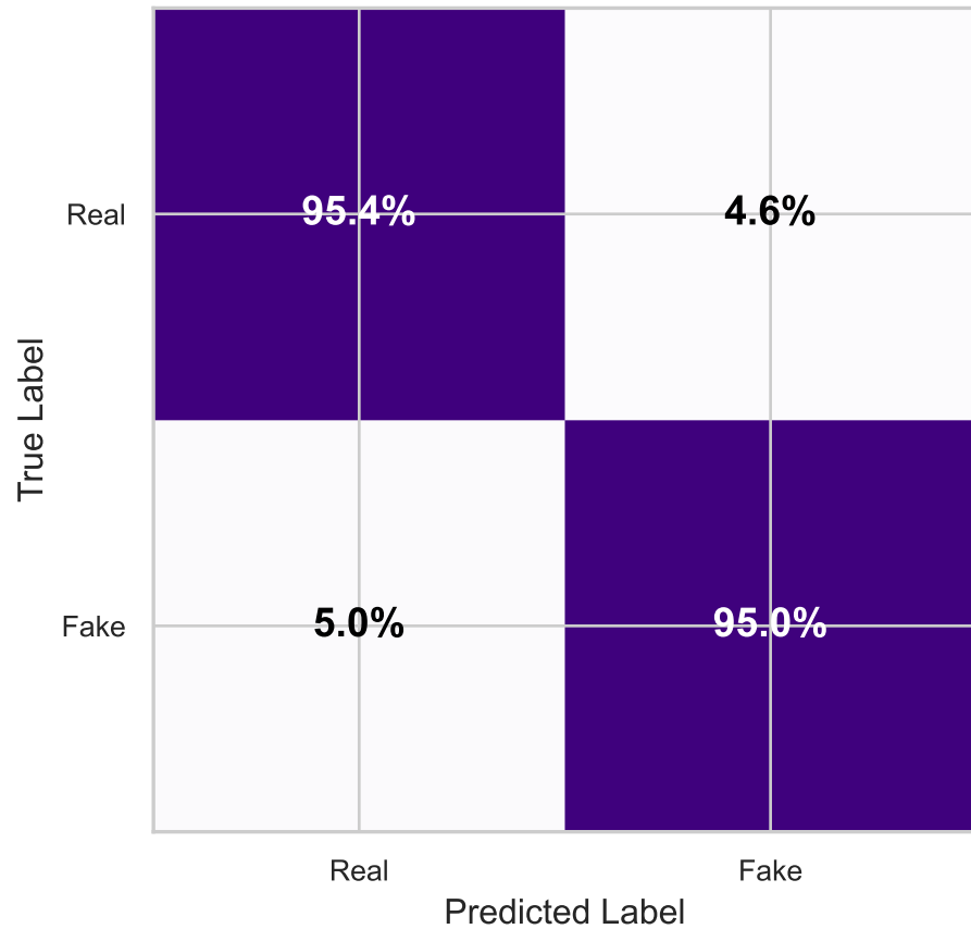
Confusion Matrix (Normalized %)
