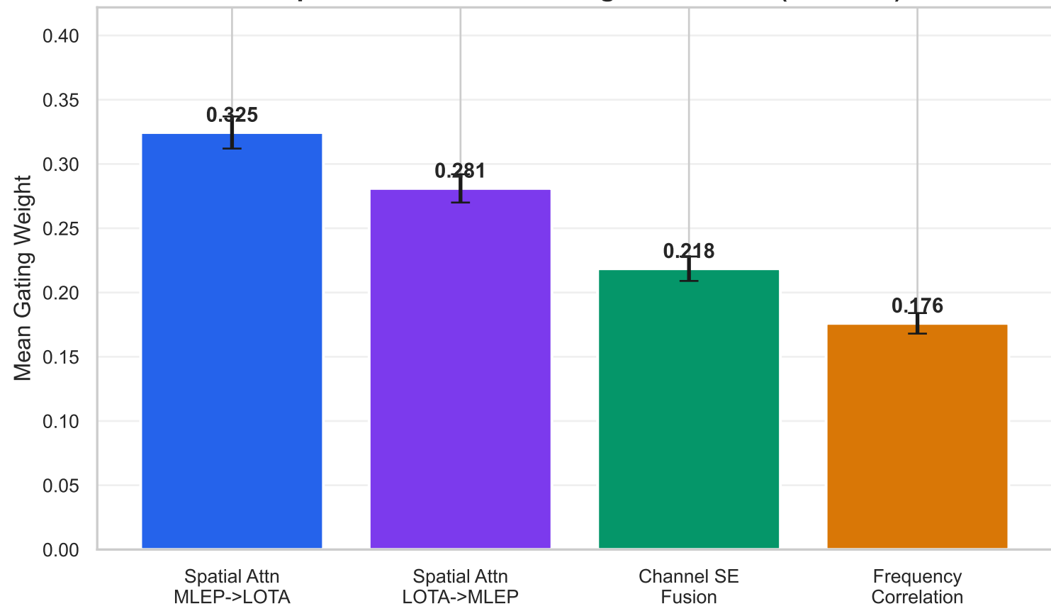
Adaptive Fusion Head Gating Distribution ( \tau = 0.5 )
