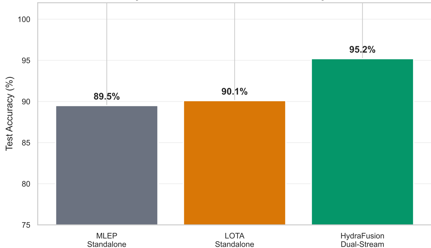
Test Accuracy: Standalone Baselines vs Fused HydraFusion-Net
