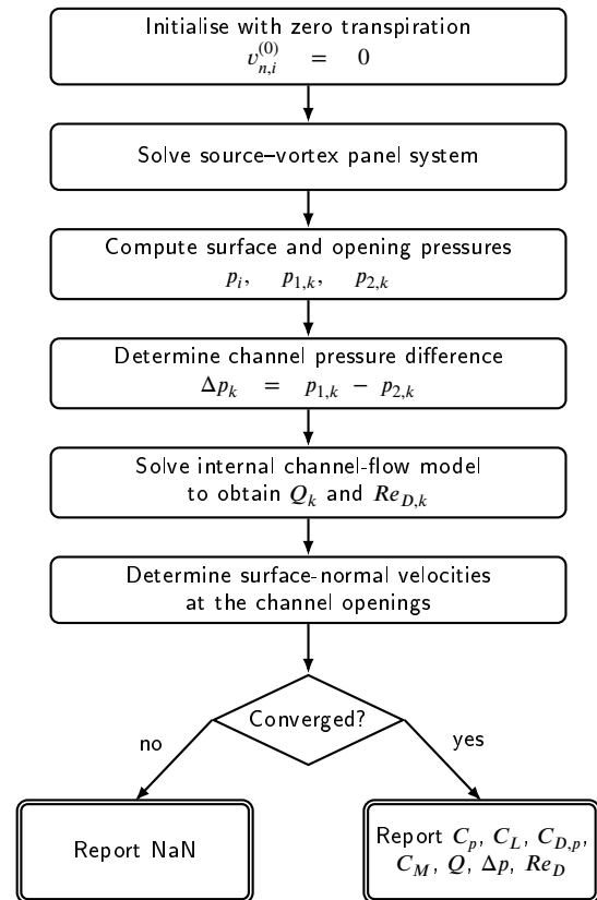
Figure 1: Coupled aero-hydraulic solution procedure.
