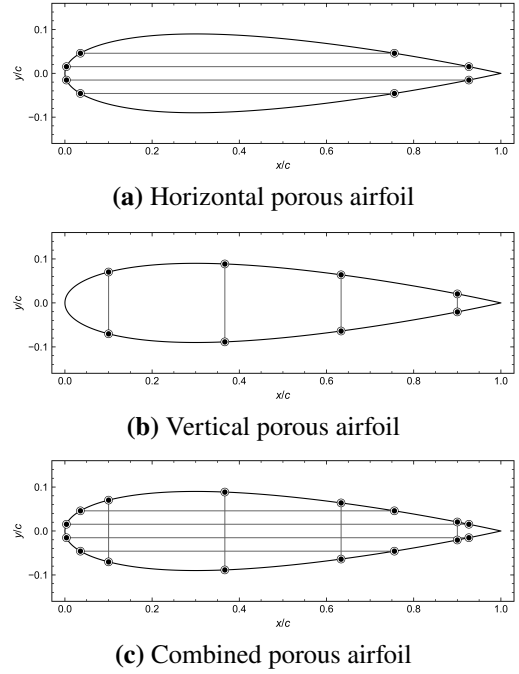
Figure 2: Internal-channel layouts considered in this study.
