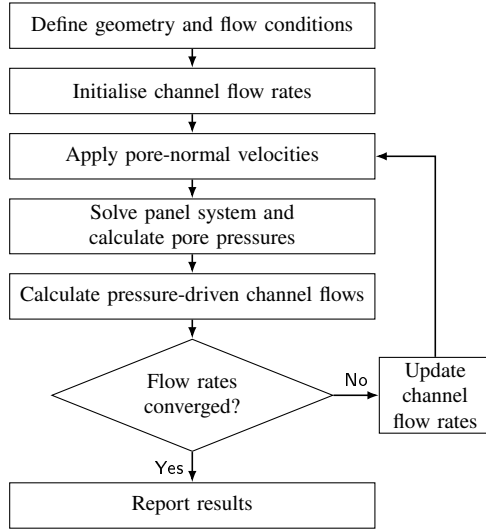
Figure 1: Coupled aero-hydraulic solution procedure. Initial flow rates are estimated from solid-airfoil pressures or a nearby converged solution. Convergence requires agreement between the current flow estimates and the pressure-driven flow rates within the prescribed tolerance.
