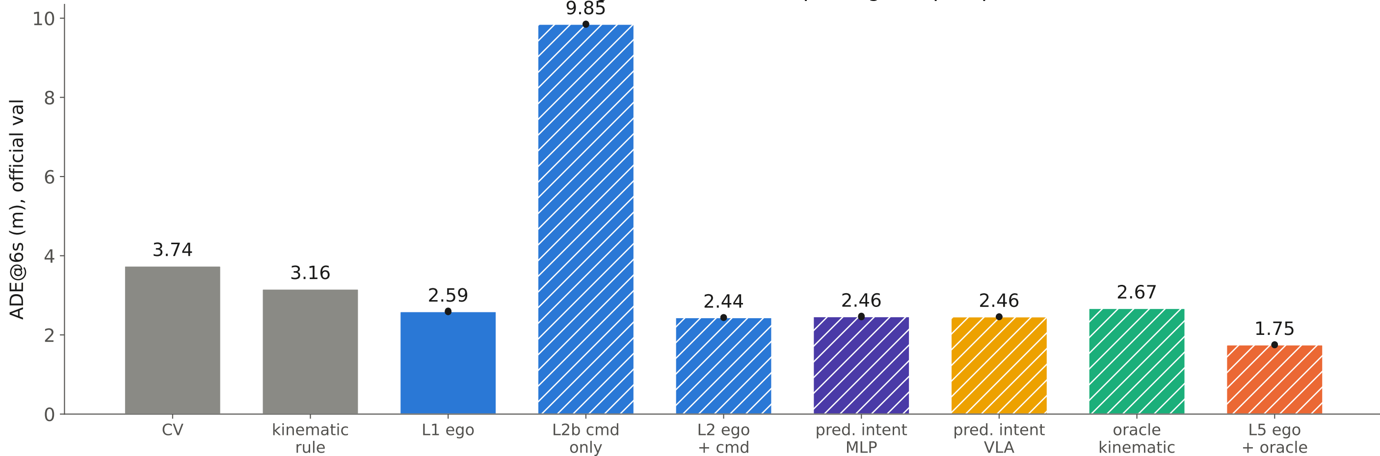
Mini information ladder on a small Ego-MLP (hatched = privileged input; pred. intent = C7 head)
