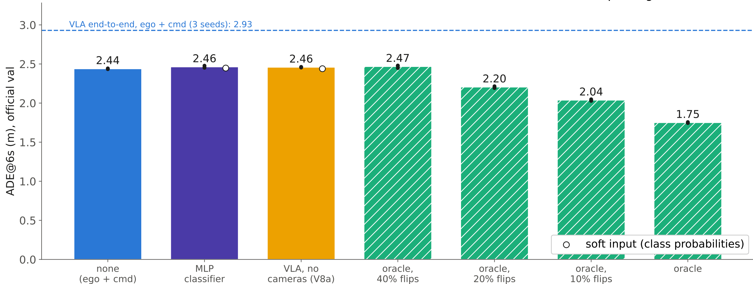
Decision bottleneck: one fixed head, different meta-action sources (hatched = privileged)
