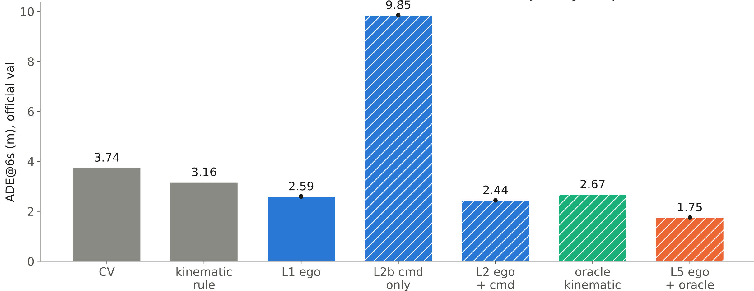
Mini information ladder on a small Ego-MLP (hatched = privileged input)
