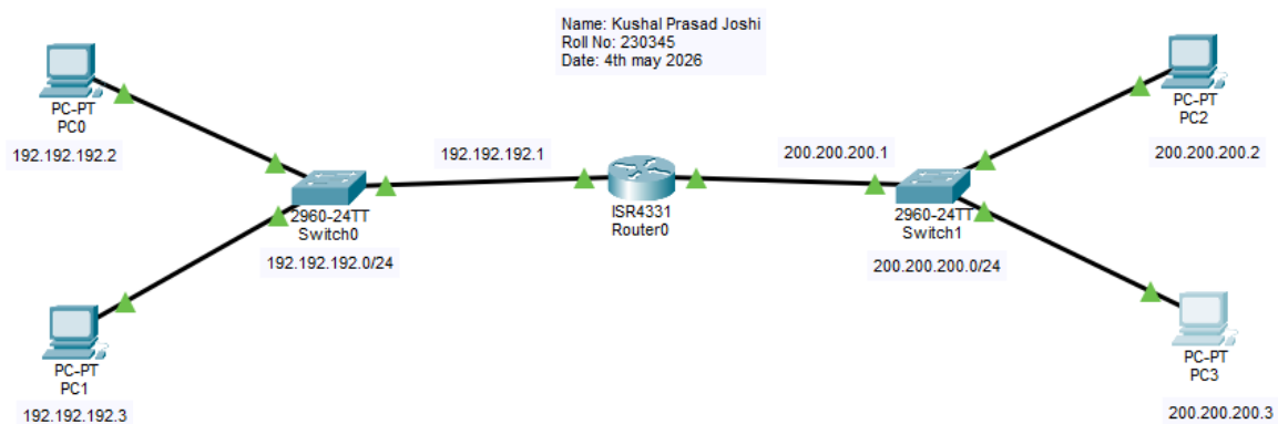
Figure 2: Configure Switch and Router with CLI practice
