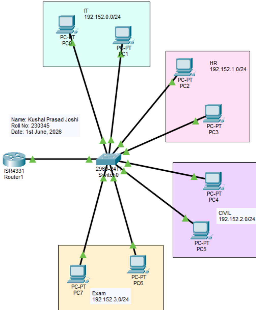
Figure 1: Multiple VLANs on single switch
