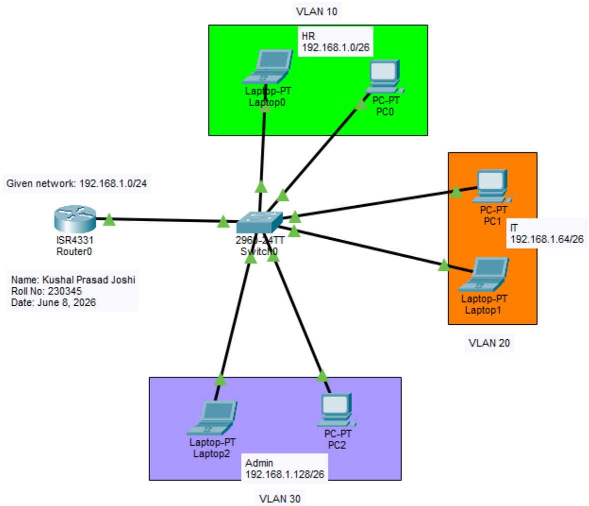
Figure 1: DHCP Configuration with 3 VLANs
