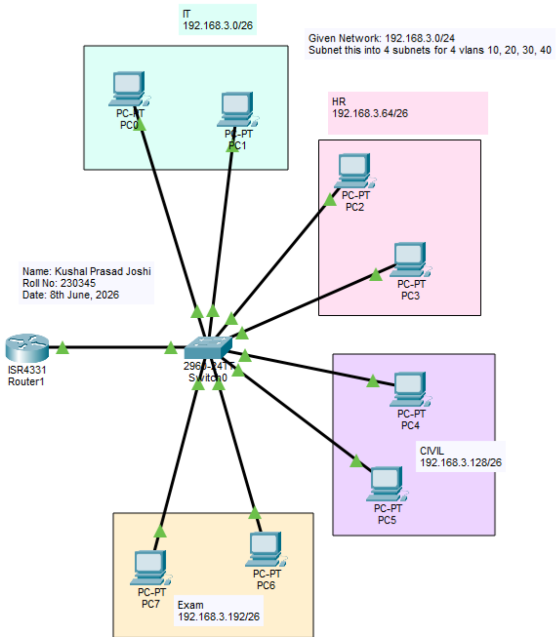
Figure 2: DHCP Configuration with 4 VLANs
