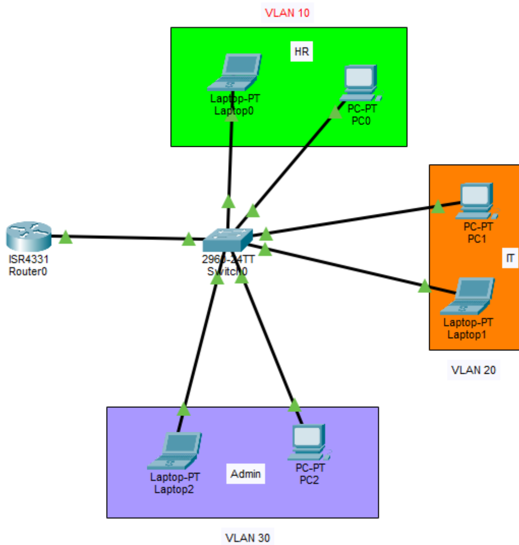
Figure 1: Virtual LANs
