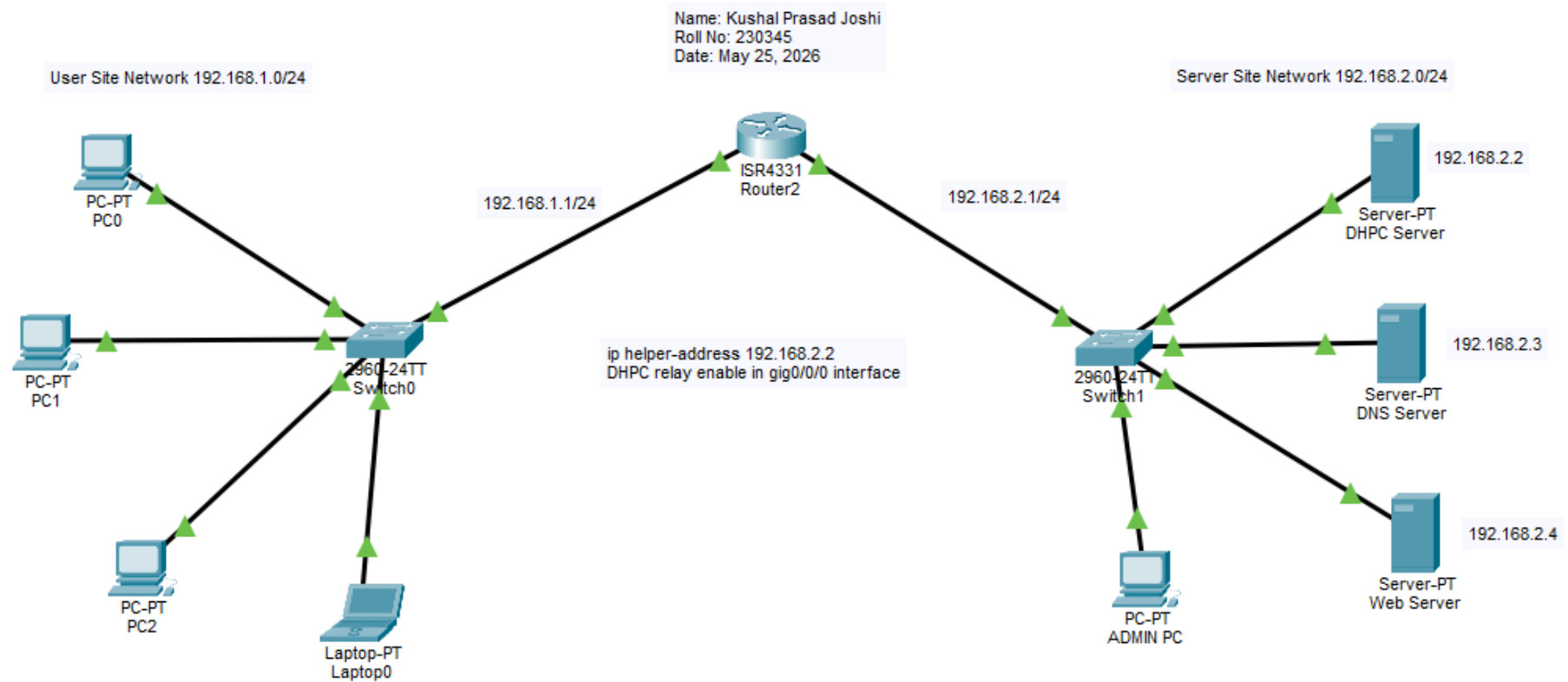
Figure 1: Configure DHCP, DNS and Web Servers
