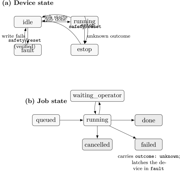
Figure 1: (a) Device state and (b) job state. The two are coupled at one point, drawn as the failed annotation: a job that fails with an unknown outcome latches the device into fault , from which there is no automatic recovery. Recovery requires safety/reset , which verifies the instrument before returning it to idle . waiting_operator allows an instrument whose steps are performed by a person to participate in the same job model as an automated one.
