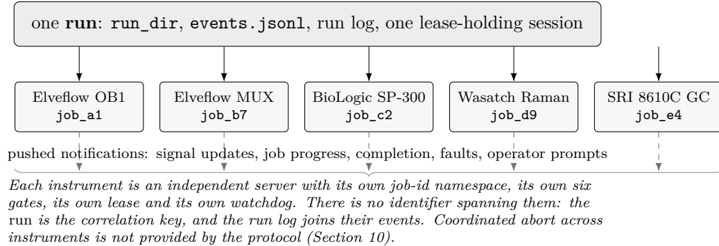
Figure 3: A five-instrument electrochemistry experiment. The composition is horizontal rather than hierarchical: no instrument knows about any other, and the orchestrating run holds one lease per device from a single session. This keeps each device’s safety envelope independent and local, at the cost of leaving cross-device atomicity to the run script.
