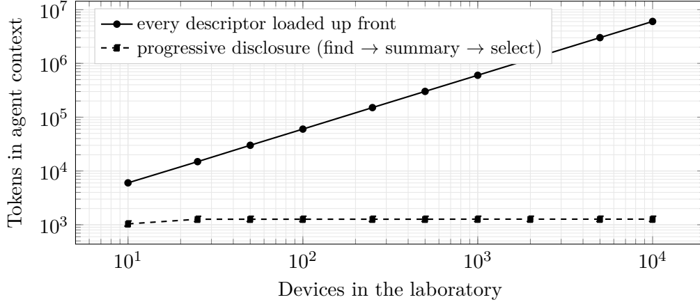
Figure 5: Context cost against laboratory size. Naive loading grows linearly with device count, exceeding six million tokens at 10,000 devices. The progressive path is effectively flat at roughly 1,270 tokens, because the agent reads five cards, one summary and two selected specifications regardless of how many instruments exist. Token counts use the proxy described in Section 9.
