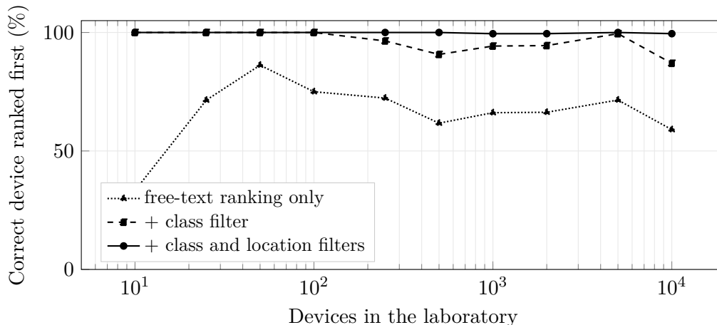
Figure 6: Retrieval under growth, 200 trials per point. A query states a task and a bay; a trial succeeds when the first result is an instrument of the class that performs the task, in the requested bay. Free-text ranking alone degrades from 86% to 59% as the laboratory grows, reproducing the selection-accuracy decay reported for large tool sets [3]. The structured filters that directory/search already accepts, and that the bridge issues, hold accuracy at 99.5–100% across three orders of magnitude. The stability comes from the protocol’s structure rather than from the ranker.
