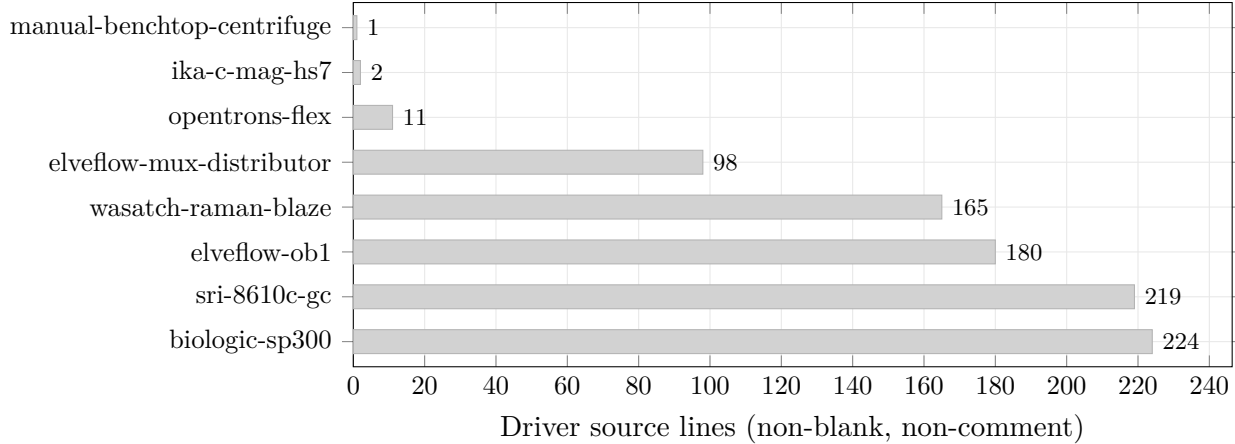
Figure 7: Integration effort per instrument, measured on the packages in supported-devices/ . The two no-code routes cost one and two lines: a human-operated centrifuge is driven entirely by operator prompts, and the IKA hotplate by declared serial commands, with the behaviour expressed in descriptor.yaml rather than in Python. Wrapping an existing ecosystem costs eleven lines through the PyLabRobot adapter. Only instruments reached through a proprietary vendor SDK require a substantial driver, between 98 and 224 lines. The safety envelope, detail tiers, jobs and notifications are inherited in every case.
