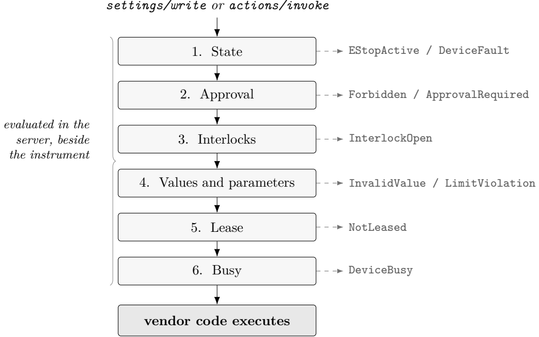
Figure 4: The six gates, evaluated in this fixed order on every write and invocation. Each gate has exactly one refusal, shown on the right. Vendor code runs only when all six pass. The order is normative because it determines which refusal an agent observes first, and therefore what it can learn from being refused. Every gate is evaluated on the device side of the network, so the enforced envelope does not depend on the model’s context, prompt, or intent.
