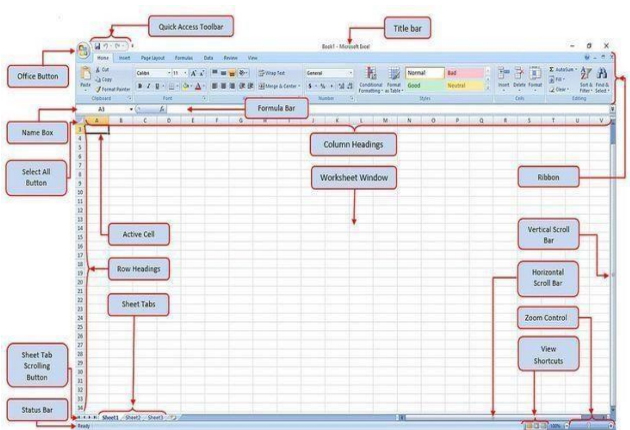
Figure 1: Structural Blueprint of the Microsoft Excel User Interface
