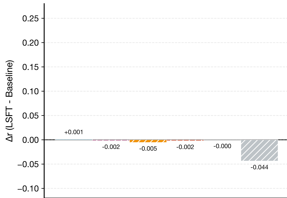
Adamson Dataset
