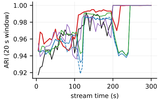
SynDrift (new clusters at 105 s, 195 s)
