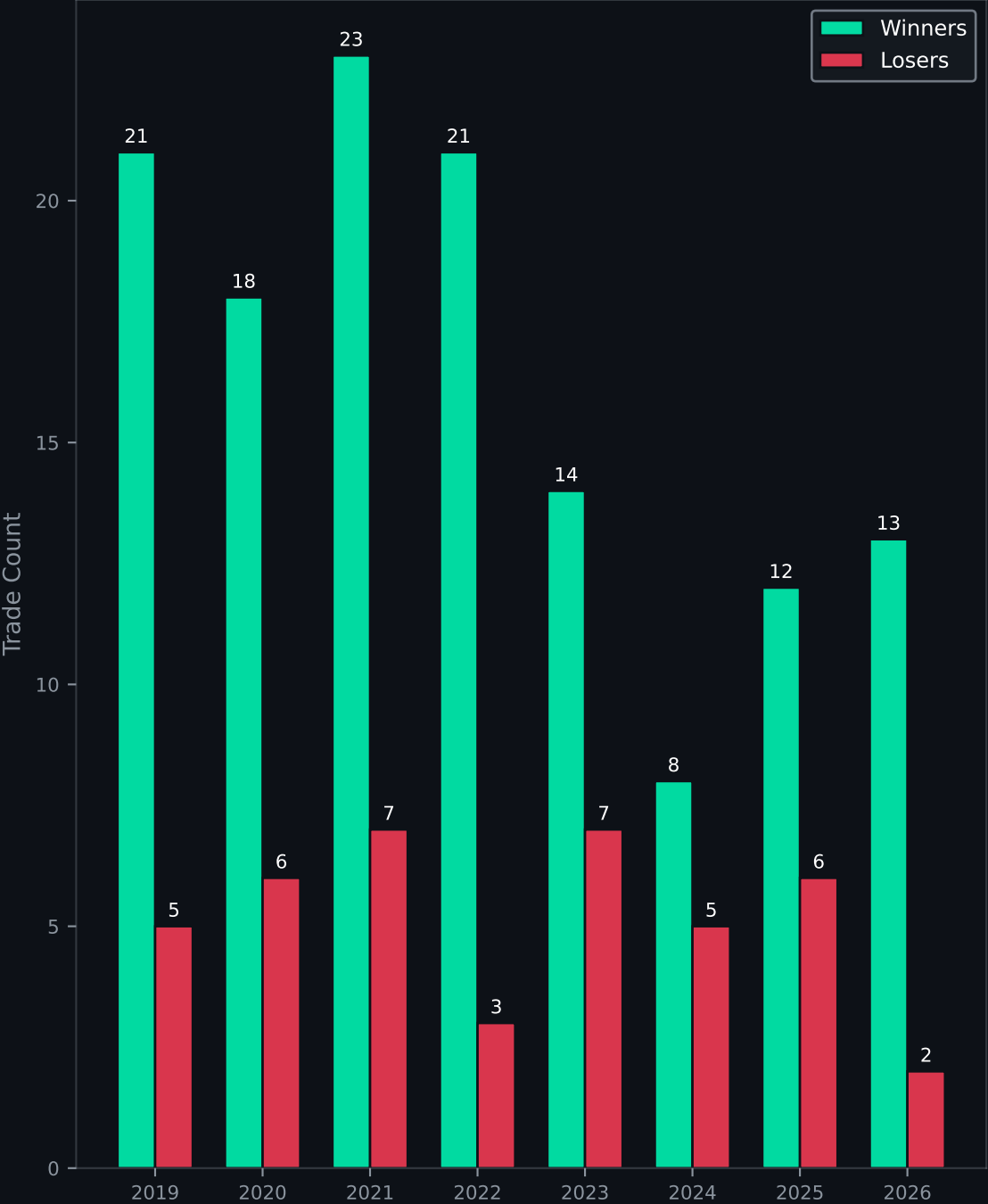
Winners vs Losers per Year (TP1=10)
