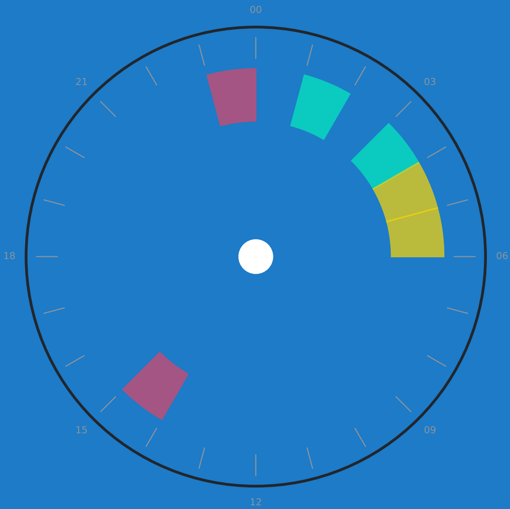
Entry Windows by UTC Hour
