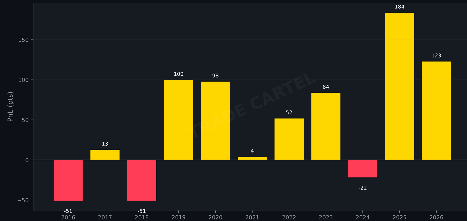
SCALP MODE — Annual PnL (ATR≥6+TP=30)
