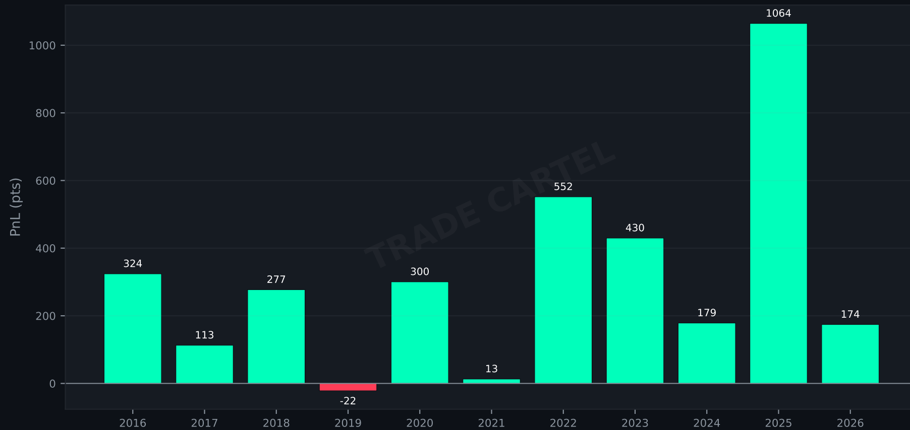
TREND MODE — Annual PnL
