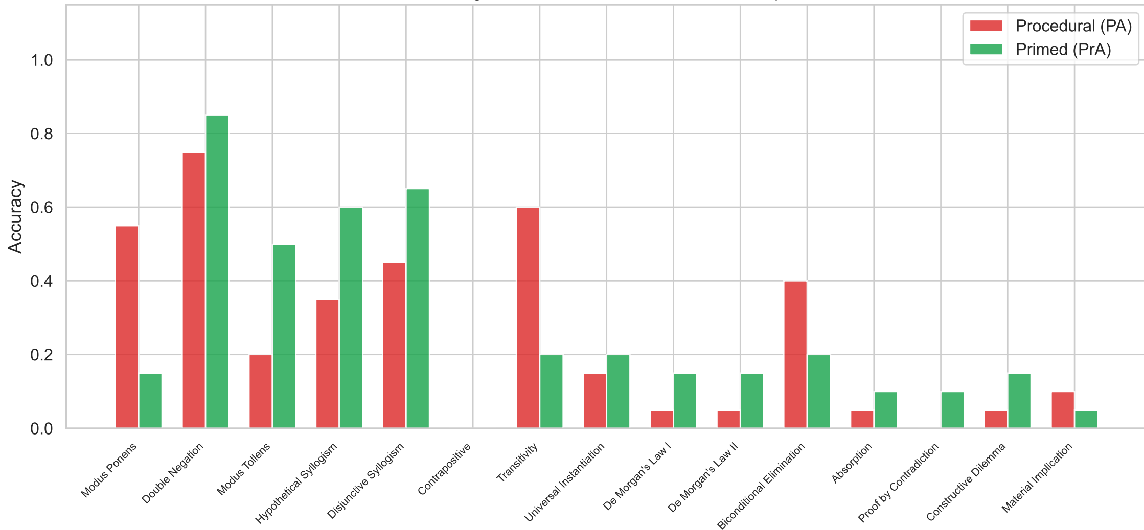
Priming Effect: Does a Rule Reminder Help?
