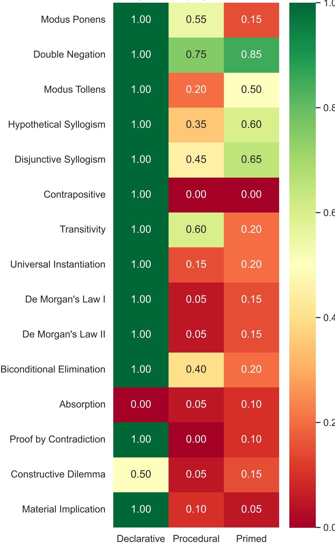
Accuracy Heatmap by Rule × Condition
