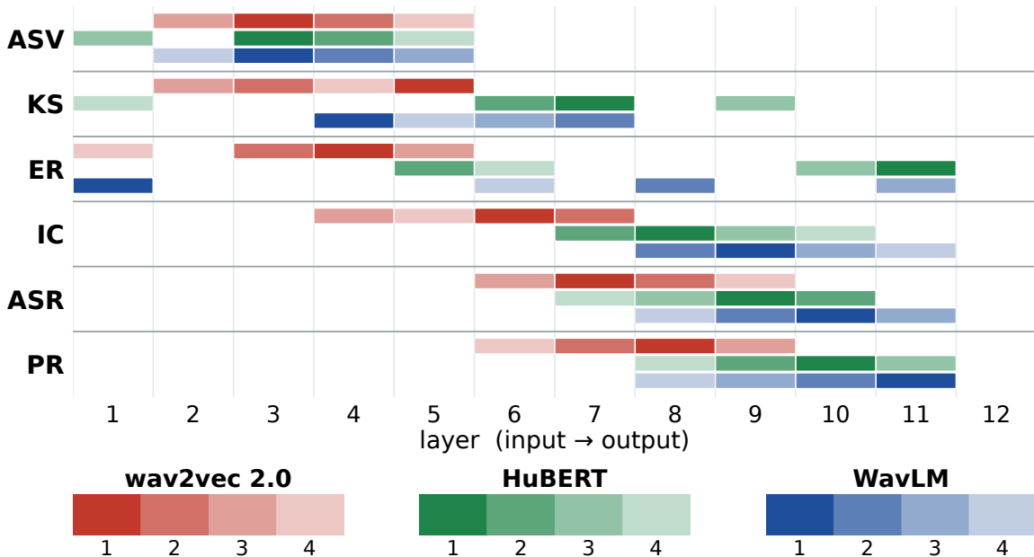
Top-4 quantization-sensitive layers per task (2-bit GPTQ)
