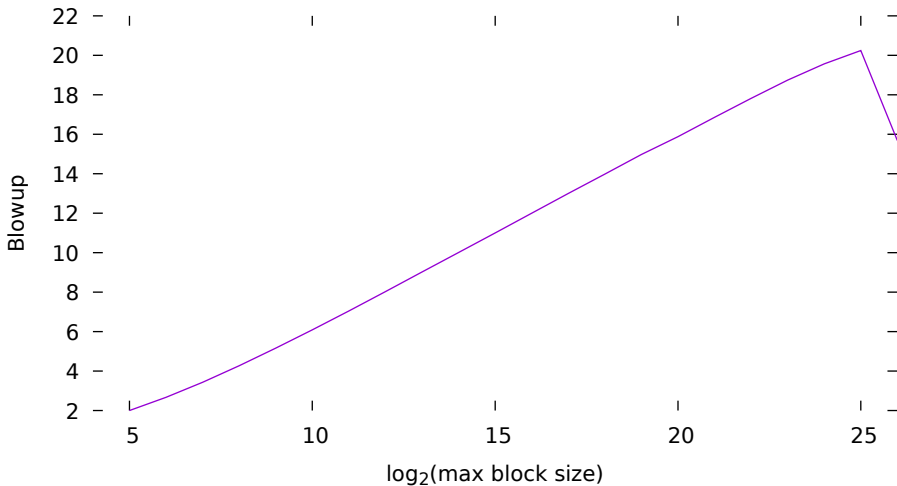
Bump allocator blowup for worst-case first-fit workload 10^8 bytes per class
