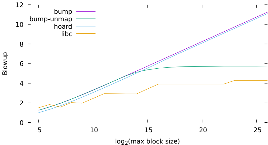
Blowup for worst-case first-fit workload 2^{27} bytes per class
