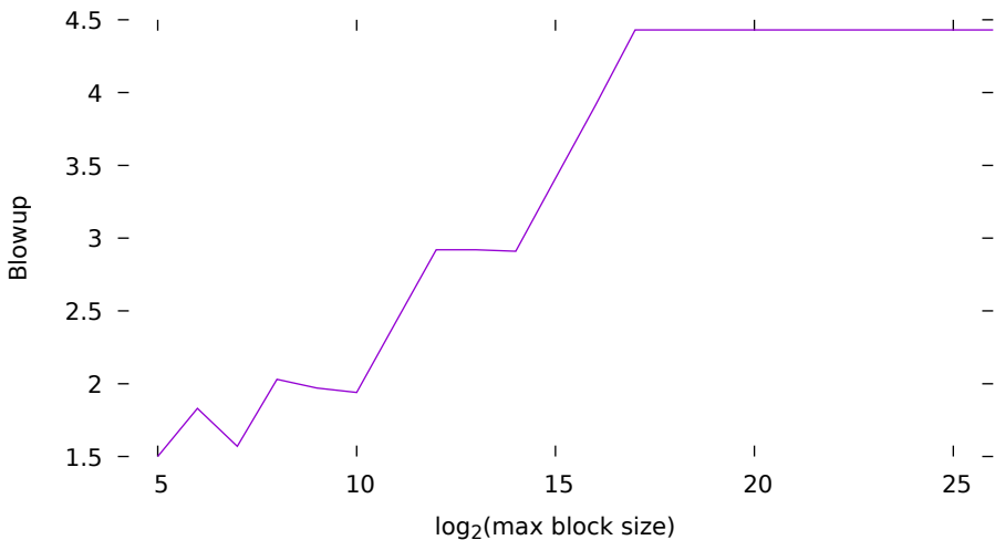
LIBC allocator blowup for worst-case first-fit workload 10^8 bytes per class
