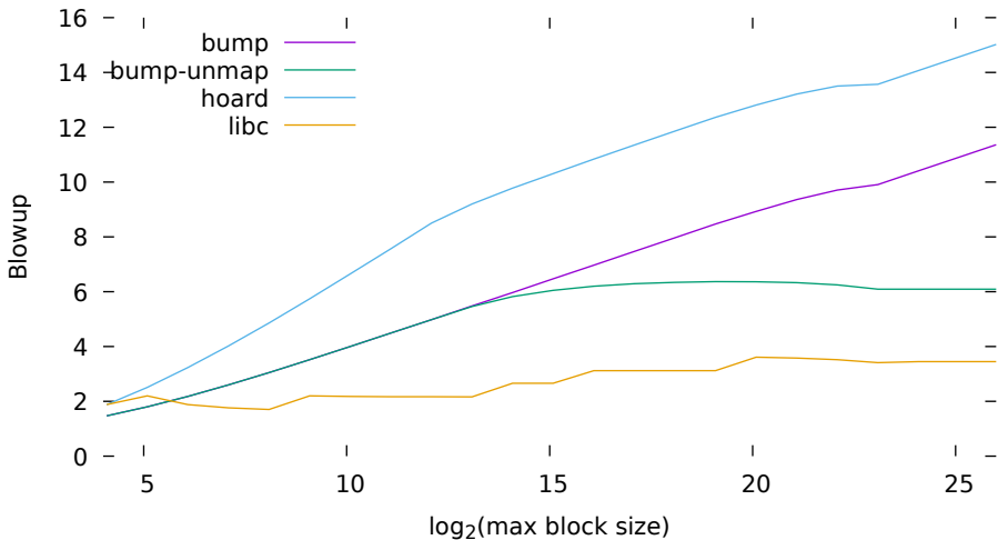
Blowup for worst-case first-fit workload 10^8 bytes per class (min block size=17)
