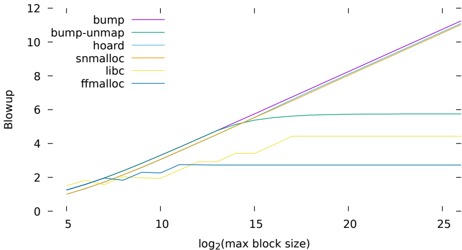
Blowup for worst-case first-fit workload 2^{27} bytes per class (min block size=32)
