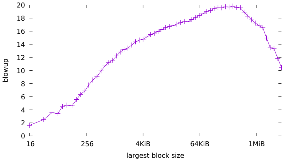
Blowup for the worst-known Hoard workload
