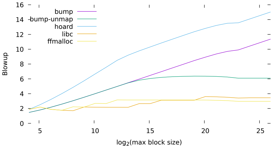
Blowup for worst-case first-fit workload 2^{27} bytes per class (min block size=17)
