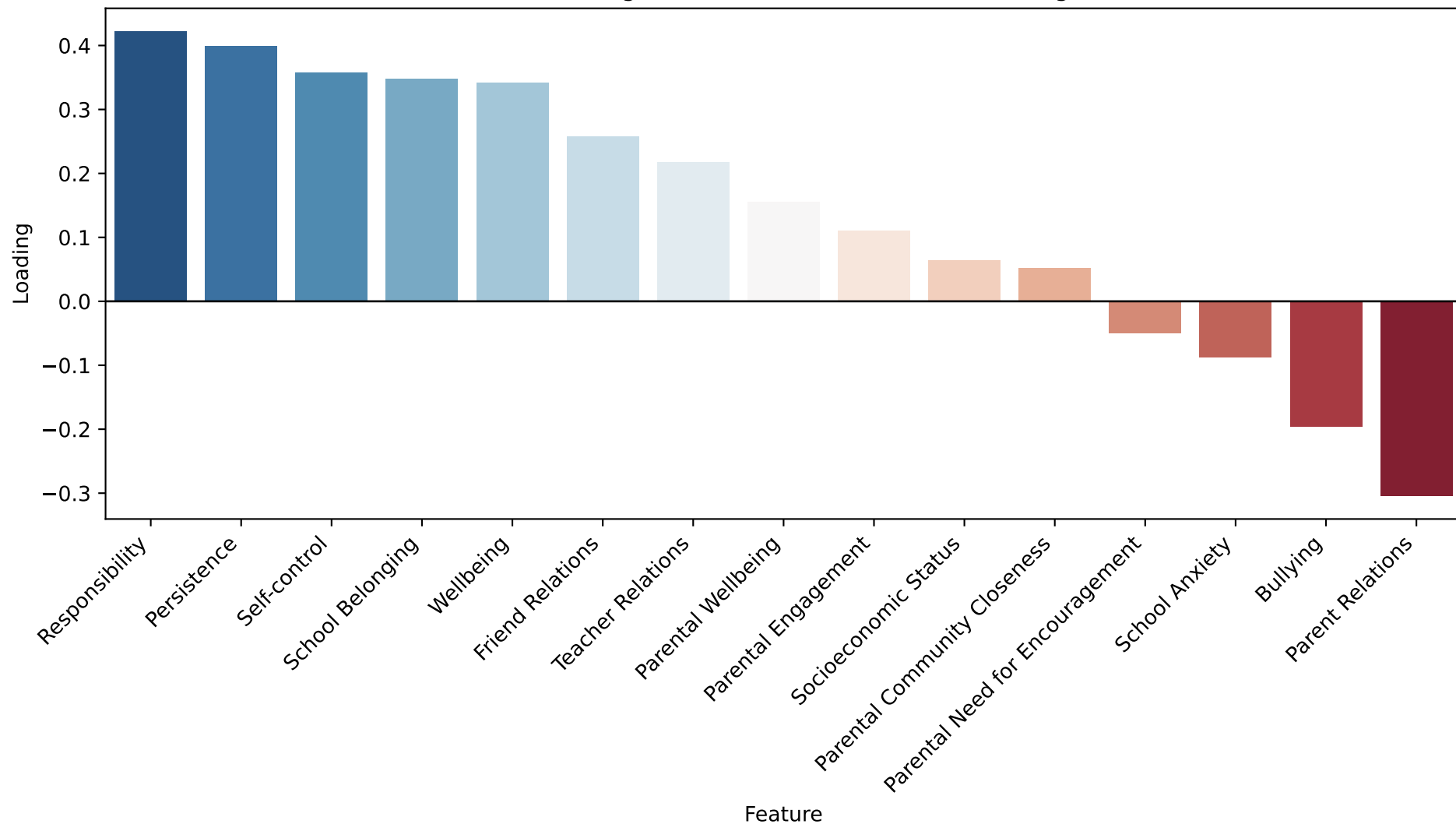
Deconstructing PCA 1: Feature Contributions (Bogota)
