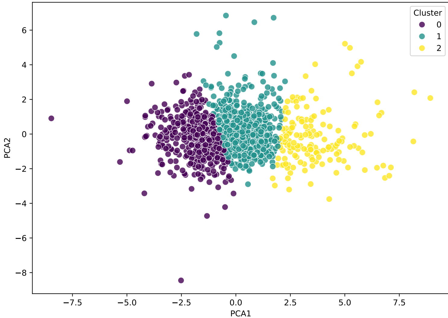
KMeans Clusters
