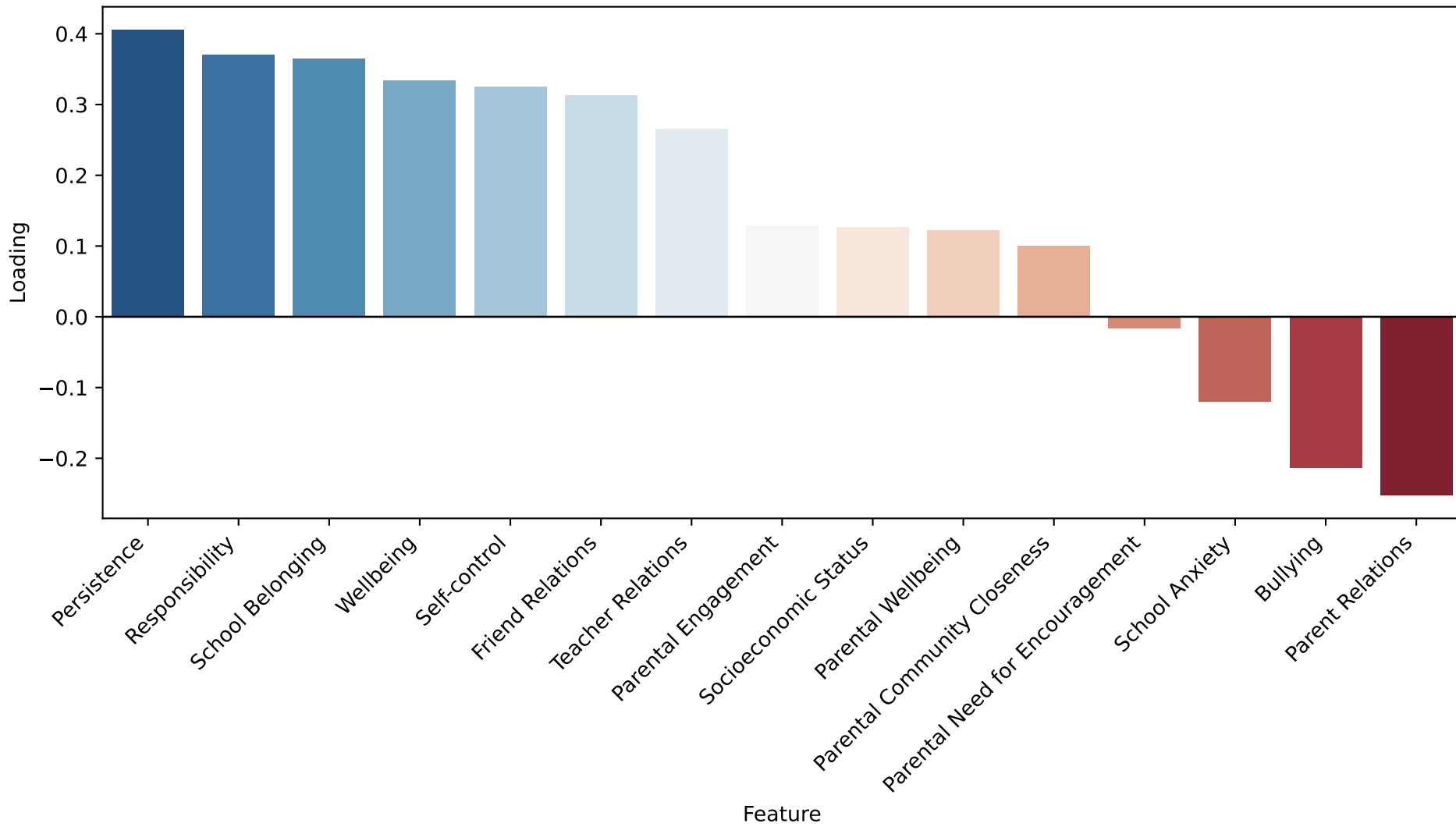
Deconstructing PCA 1: Feature Contributions (Suzhou)
