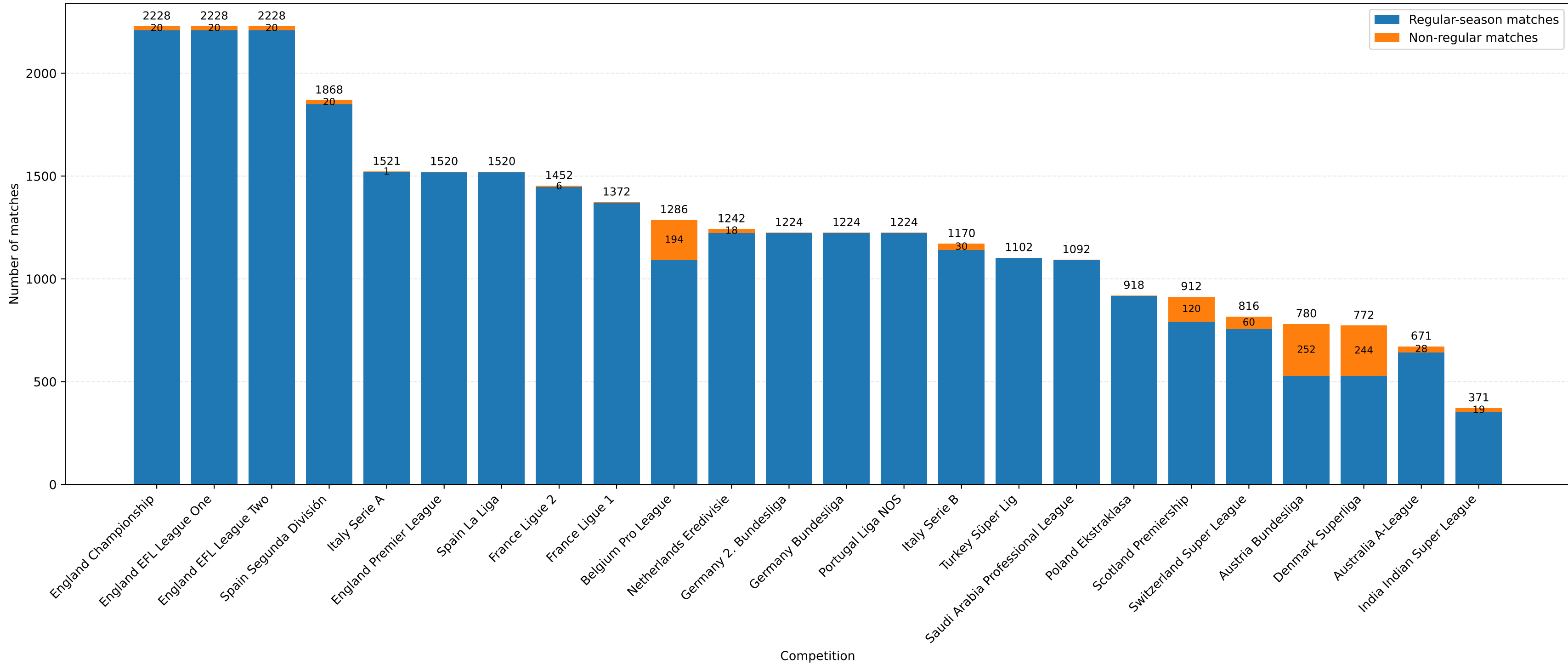
League matches per competition (2021/2022-2024/2025): regular season vs non-regular
