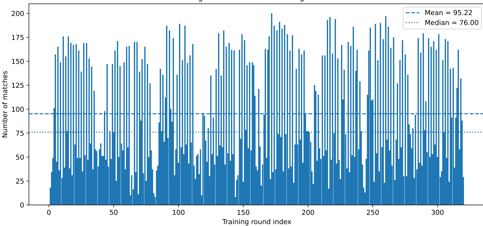
Training round sizes in chronological order
