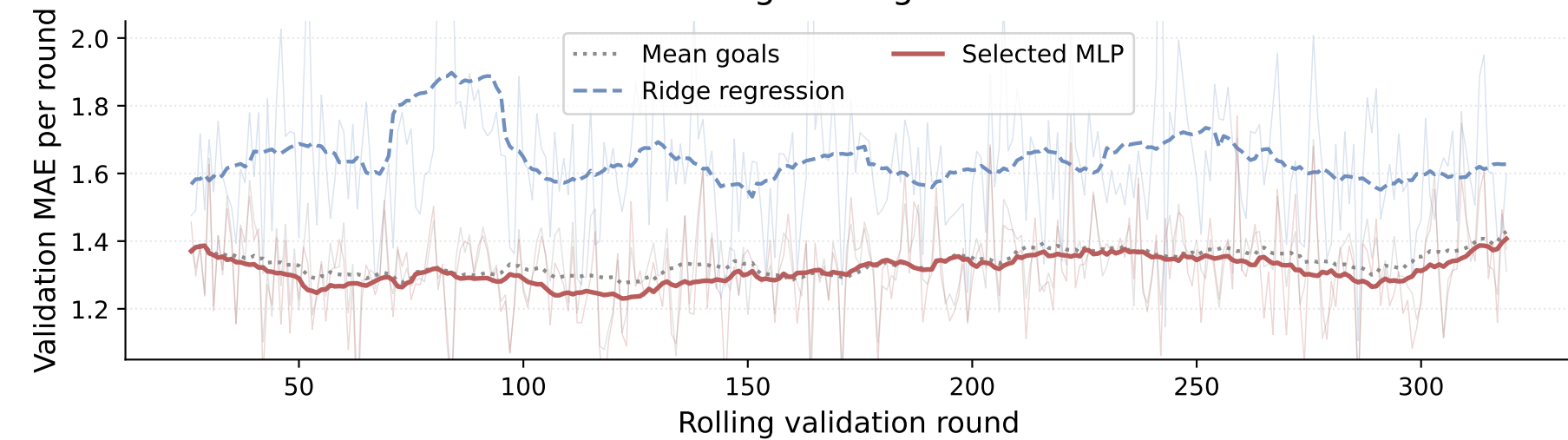
Total-goals regression
