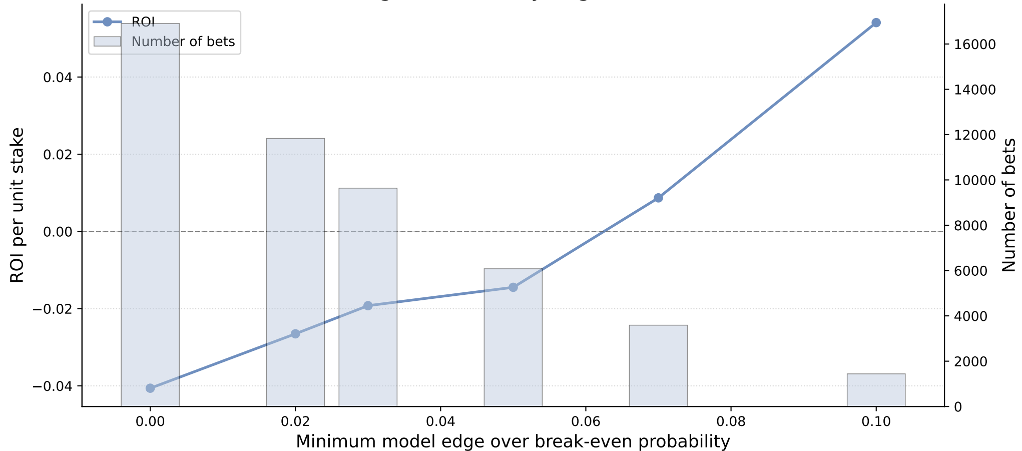
Betting simulation by edge threshold
