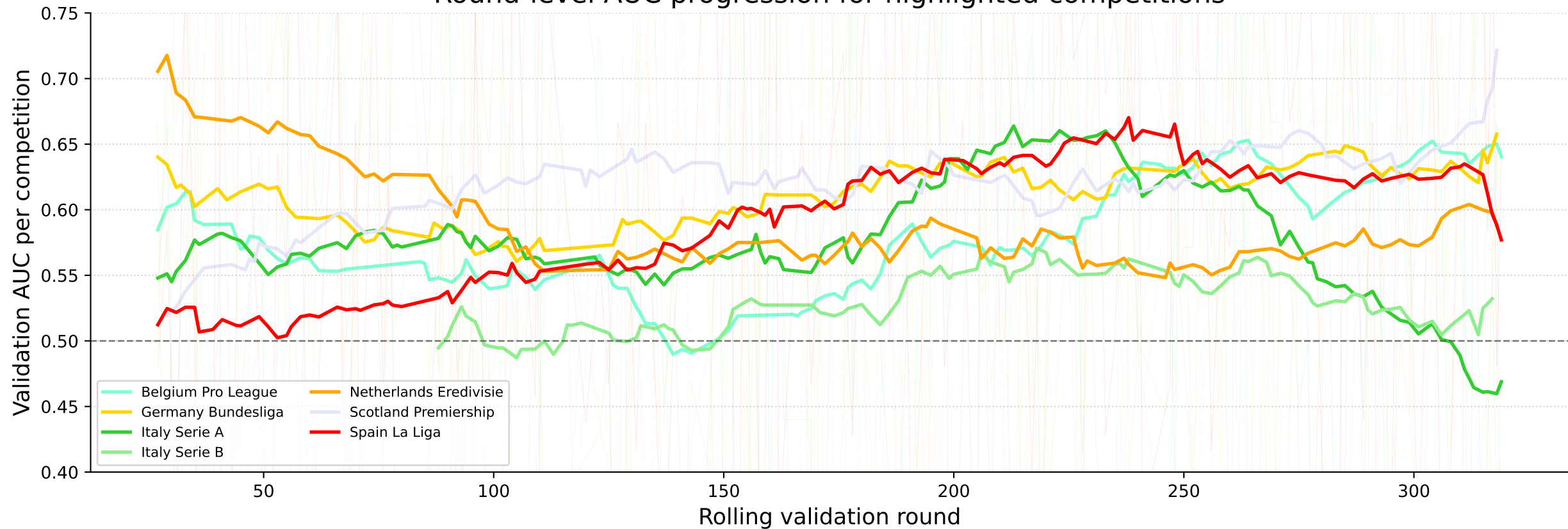
Round-level AUC progression for highlighted competitions
