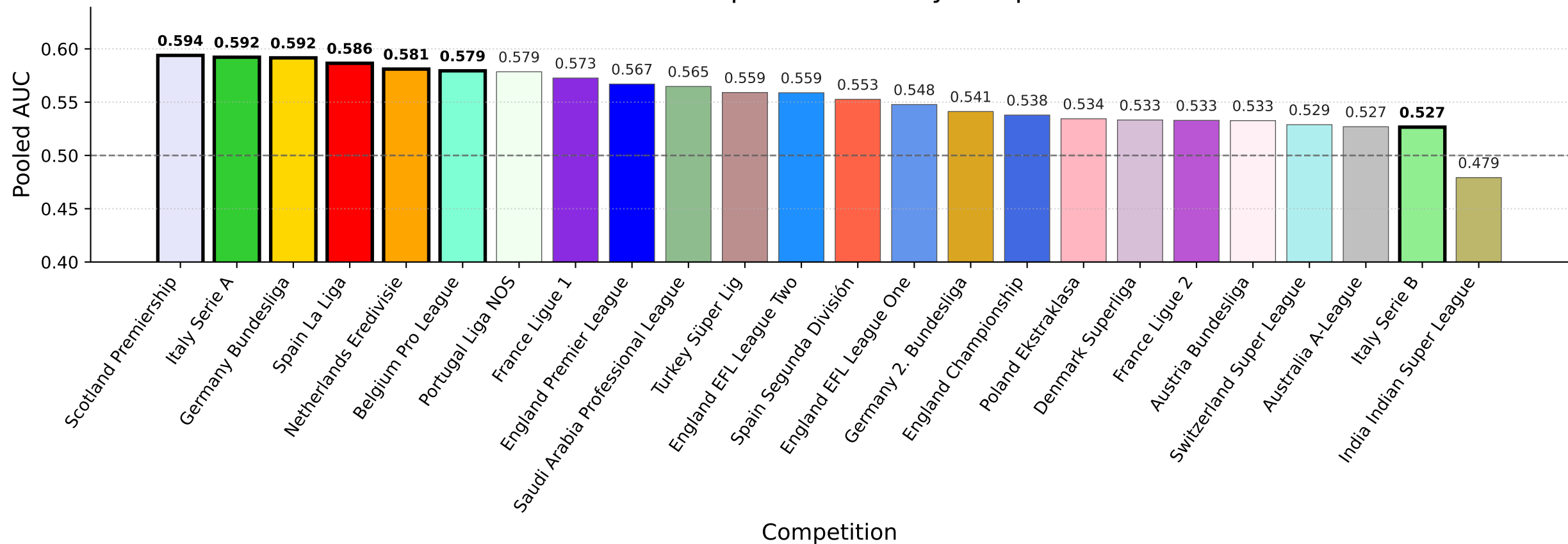
Selected MLP performance by competition
