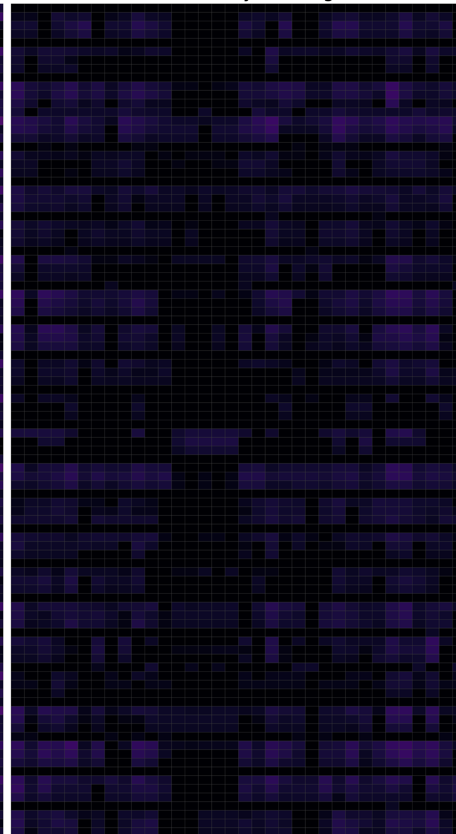
Persistently missing
