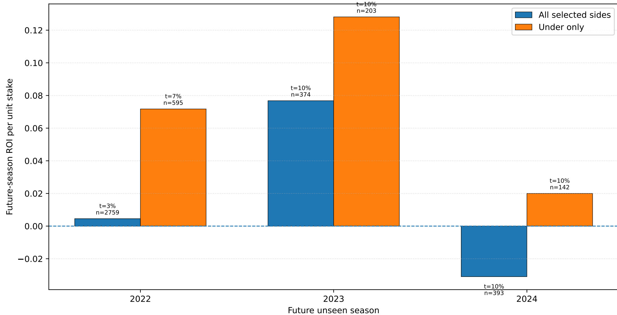
Walk-Forward Future ROI: All Sides vs Under-Only Threshold Selection
