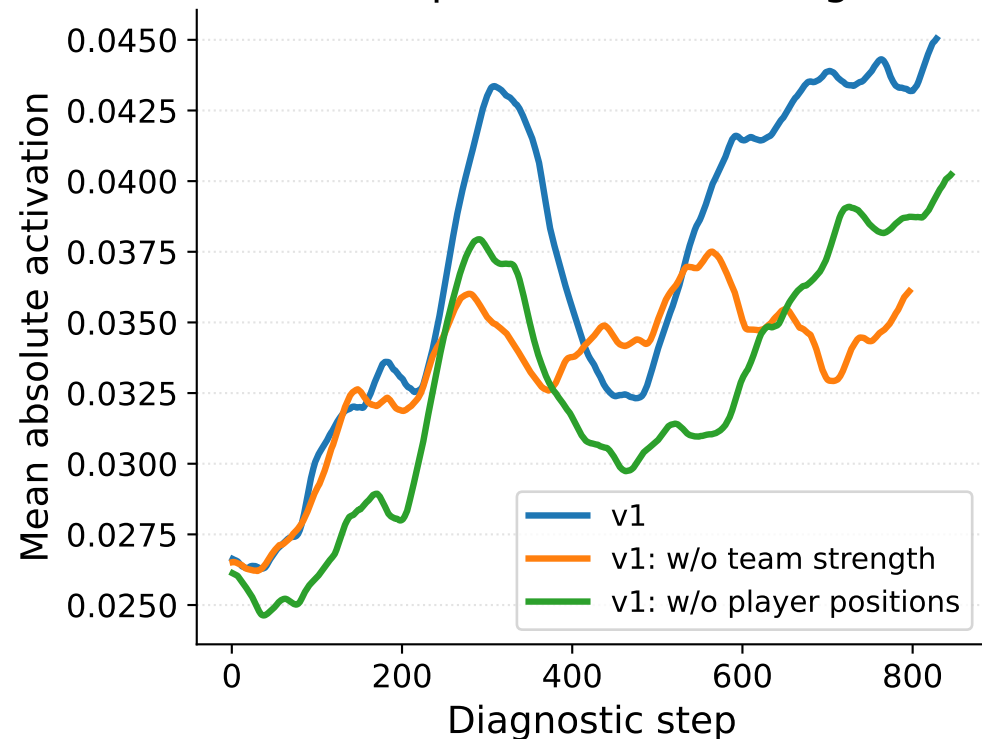
Competition Embedding
