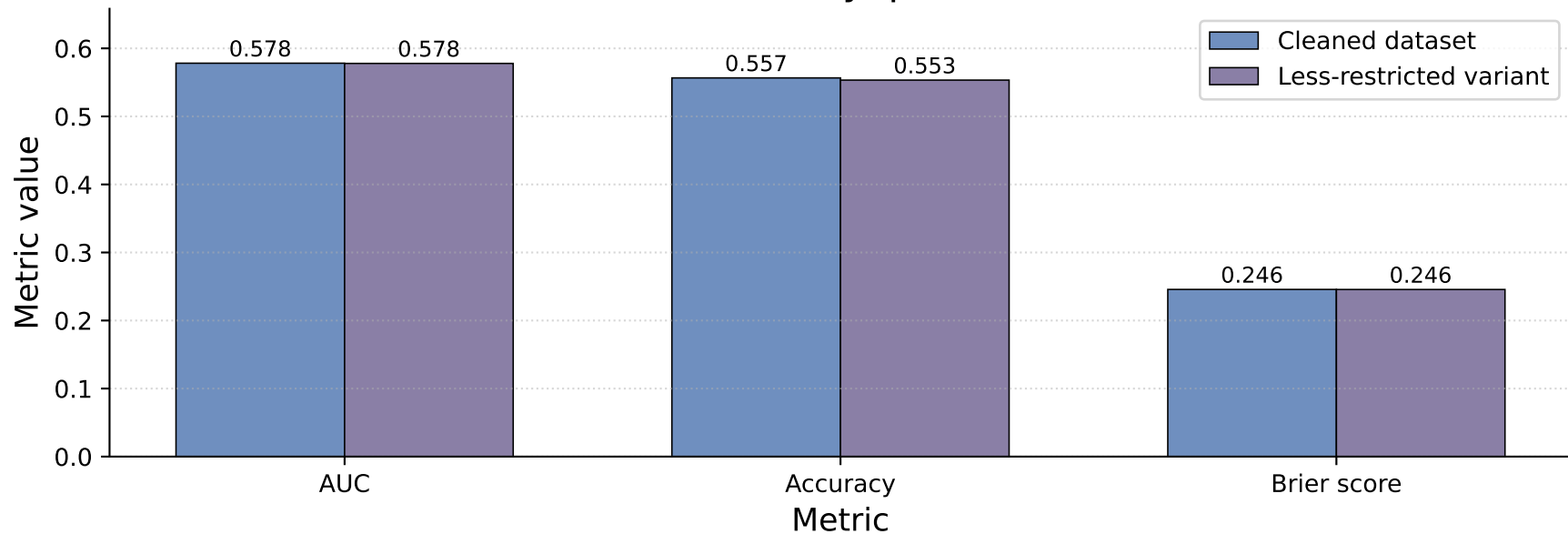
Dataset sensitivity: pooled metrics
