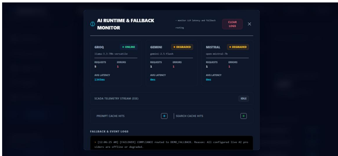
Figure: AI Runtime & Fallback Monitor auditing provider status, latencies, and circuit breakers
